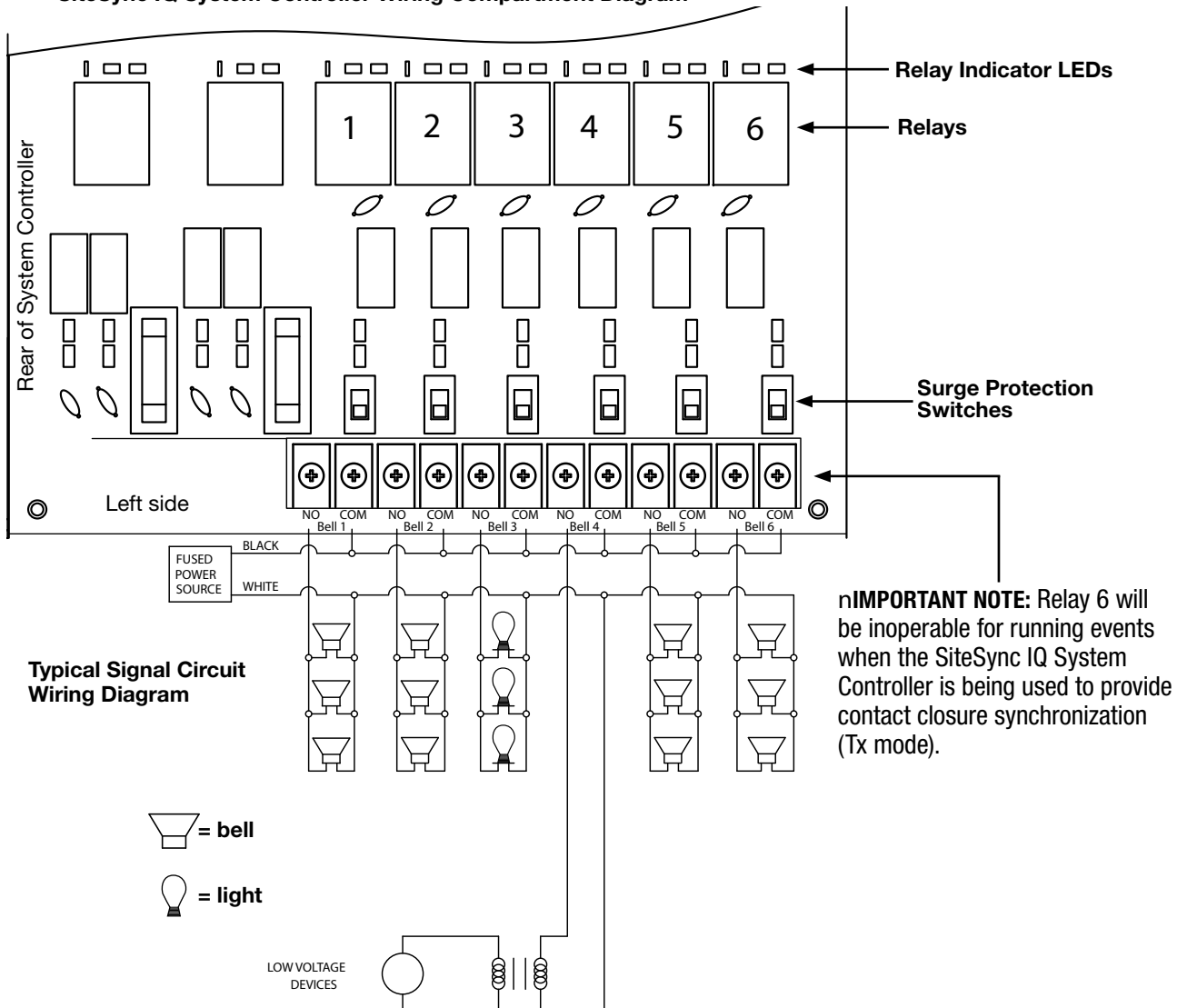
SiteSync IQ System Controller Wiring Compartment Diagram
