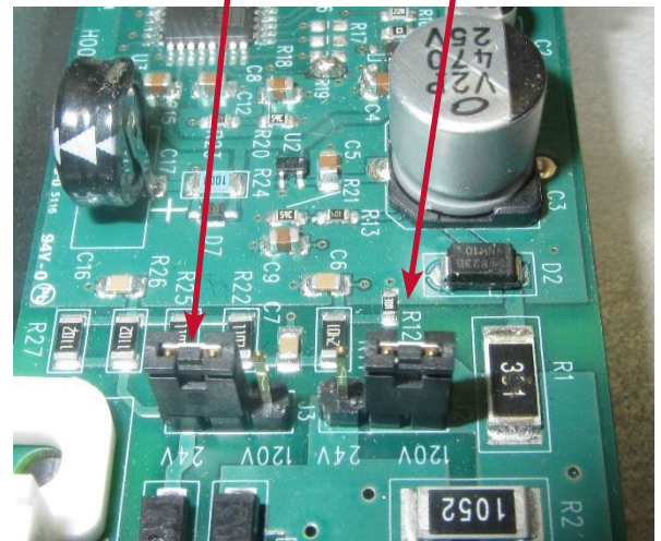
24V Correction Jumper
