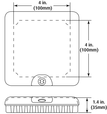
STI-9102
